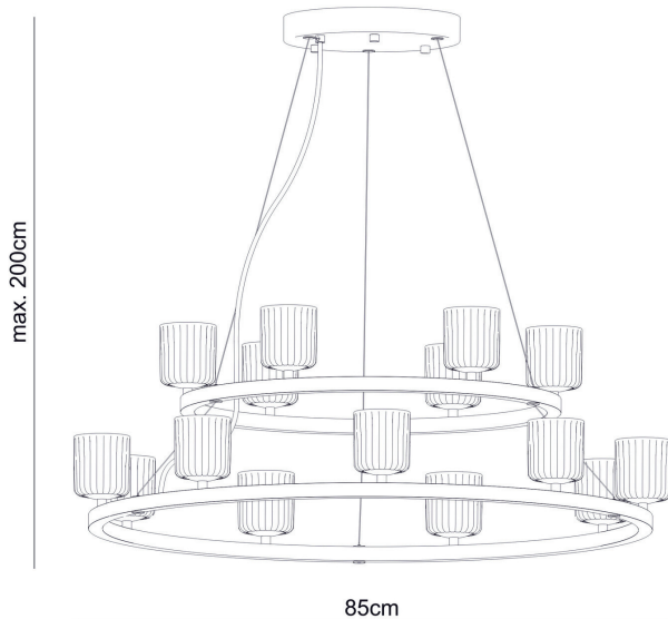
HL 6-1825/54/80 klar-Schliff
