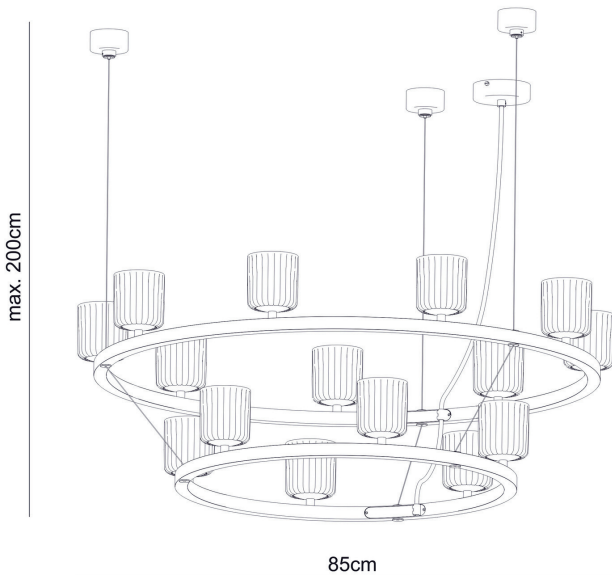
HL 6-1827/54/80 klar-Schliff
